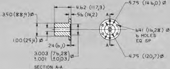
DETAIL OF COMPANION FLANGE 6L8385
