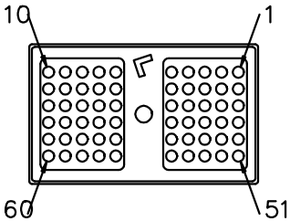
ELECTRONIC CONTROL MODULE (ECM) OEM HARENESS CONNECTOR MATING FACE (OEM端)线束60针接头
