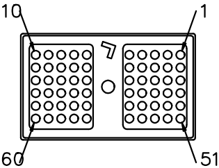
ELECTRONIC CONTROL MODULE (ECM) ENGINE HARNESS CONNECTOR MATING FACE (ENGINE端)线束60针接头
