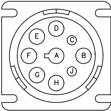
SAE J1939 DATA LINK 9-PIN SERVICE PORT CONNECTOR (OEM端)9针服务通讯接头
