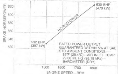
ENGINE PERFORMANCE 12V-71T WITH M95 INJECTORS
